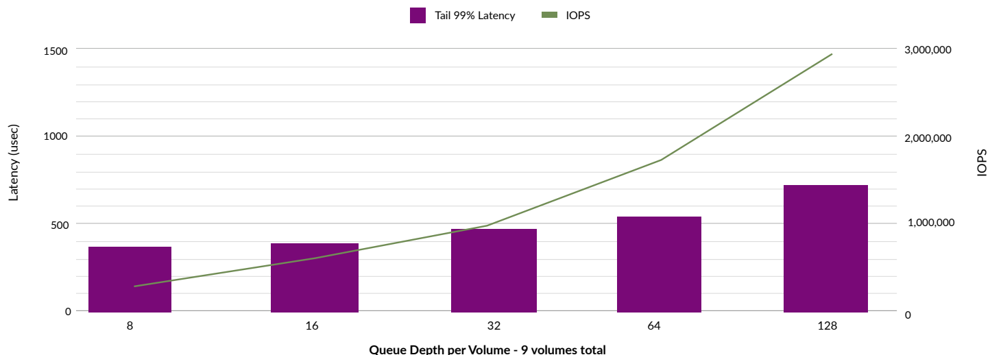
Lightbits Performance - IOPS and Tail Latency for 100% Reads
